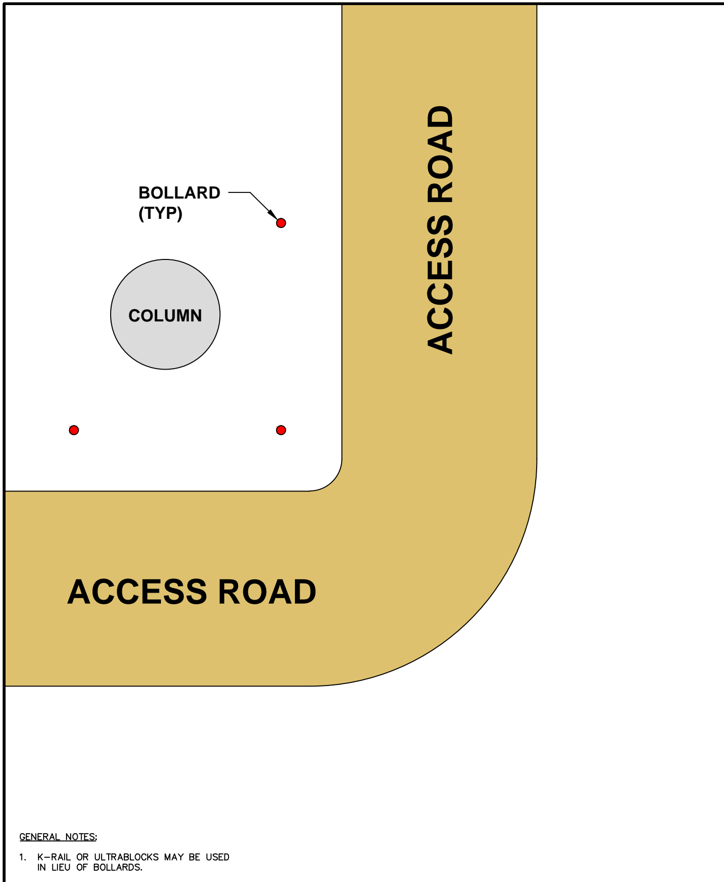
FIGURE 4 COLUMN PROTECTION EXAMPLE 4
