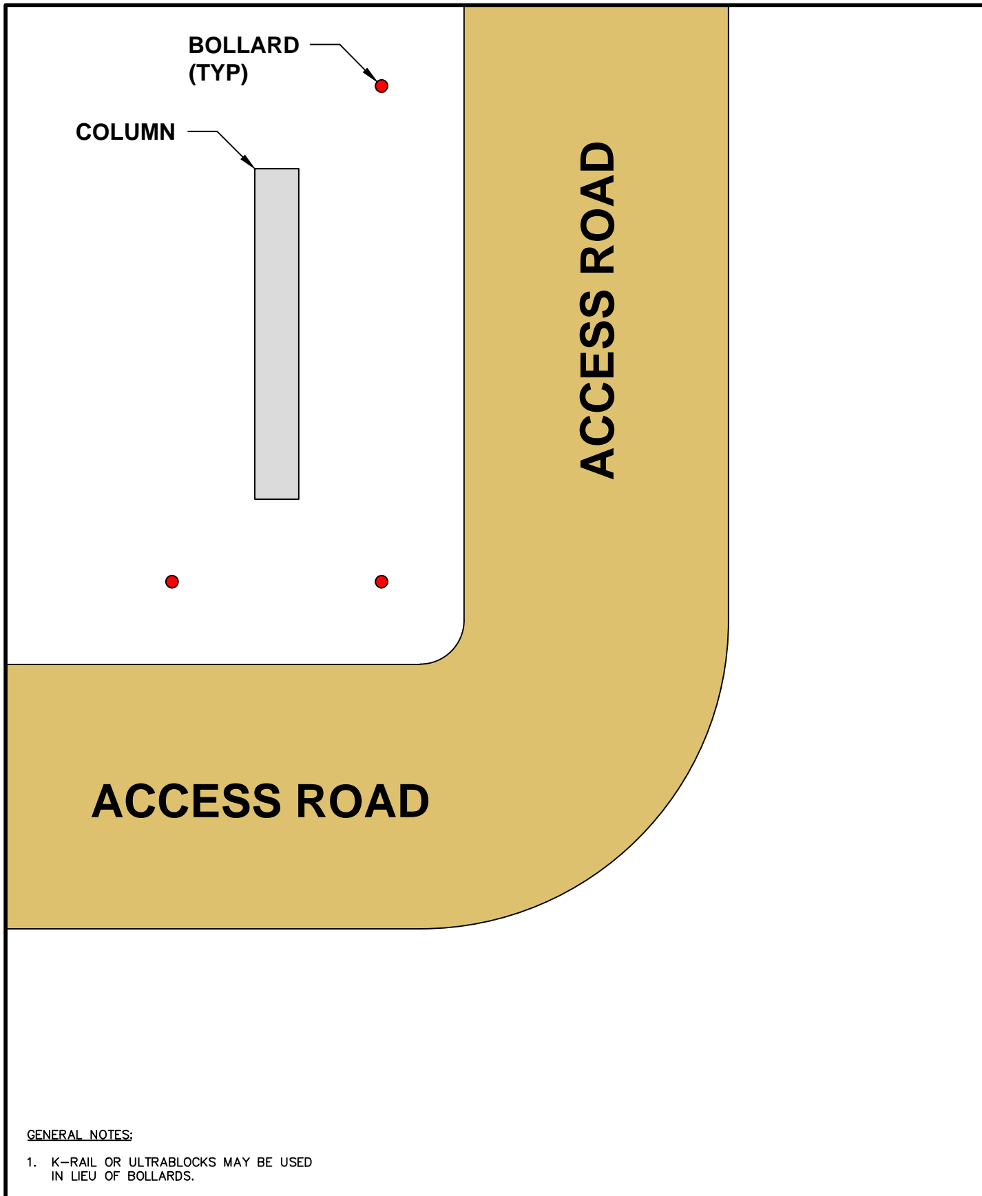
FIGURE 3 COLUMN PROTECTION EXAMPLE 3
