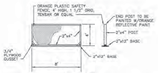
DETAIL 'B' PEDESTRIAN BARRICADE-SAFETY FENCE TYPE N.T.S.
