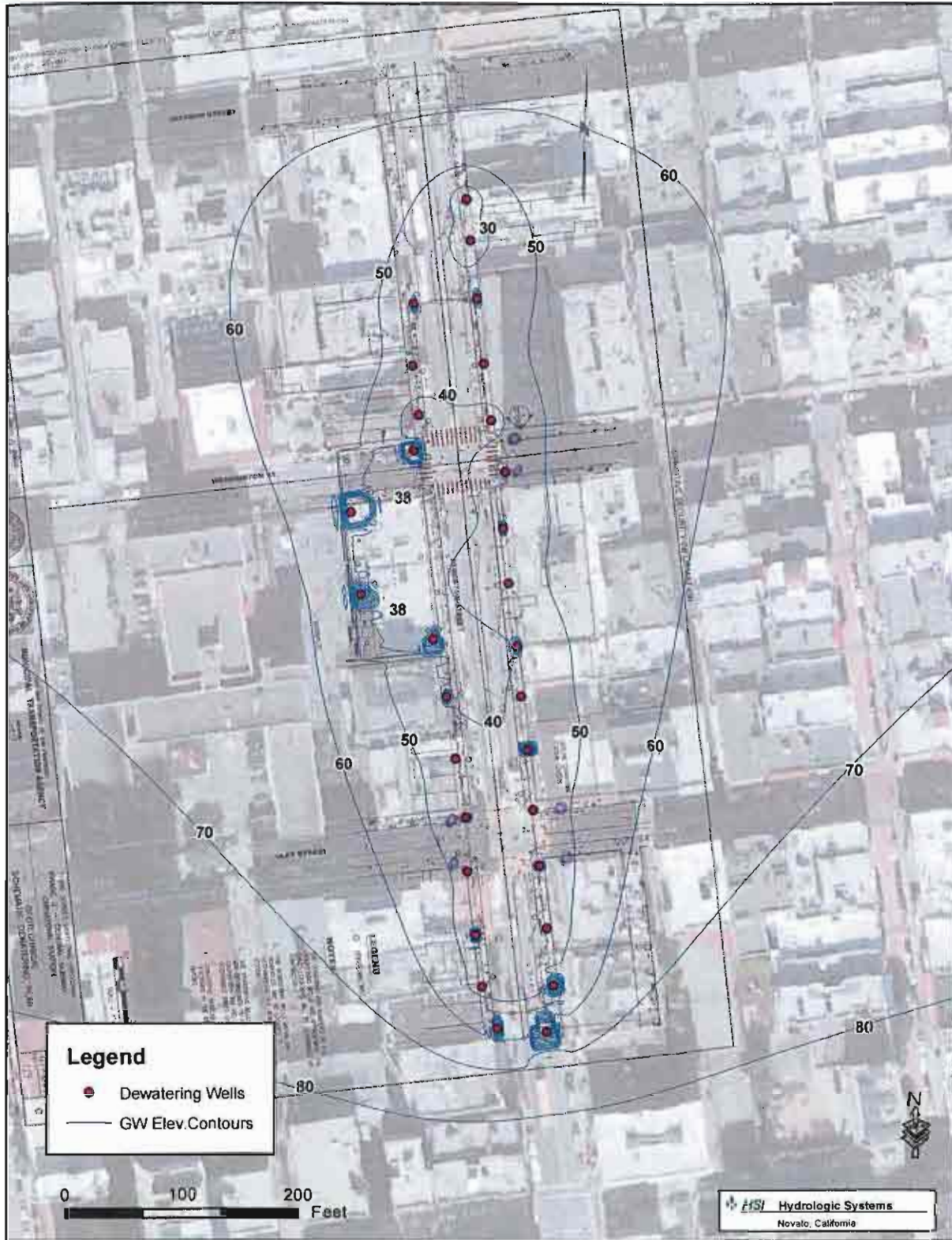
Figure ES-2. Groundwater Elevation Contours For The Equilibrium Condition. (ft. CCSF)
