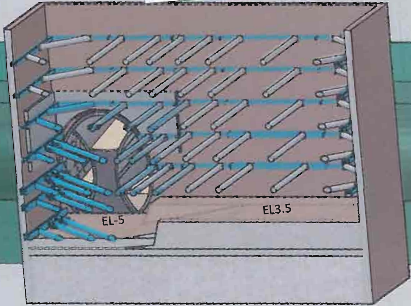
a) Cross Cut – Breakout Bench/Invert of the Side Drifts Left & Right
